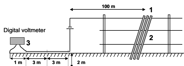
Fig. 3: Sketch of how to test a ground earth return system.
